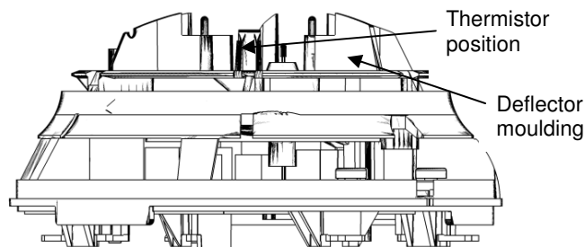
Diagram 3 - Re Assembly showing correct thermistor
