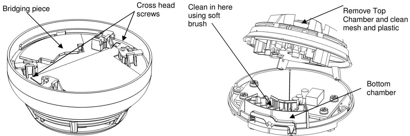
Diagram 1 - Locking bridging piece and cross head screw position
